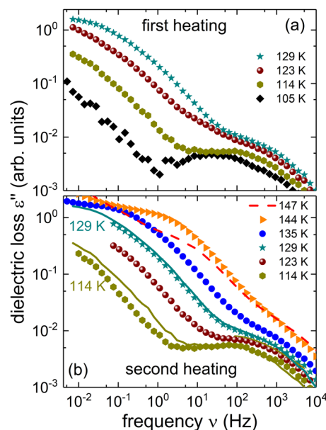
FIG. 2. Dielectric loss spectra obtained during (a) the first and (b) the second heating run performed for CO 2 -filled S x clathrate hydrate. For comparison, in panel (b), two spectra from the first heating run are included as solid lines. At 129 K, the spectra superimpose well, while at 114 K, differences are seen in the region of the main peak. The decomposition of the S x clathrate to CO 2 and hexagonal ice 37 leads to significant changes of the low-frequency part of the spectral shape, while its high-frequency part remains practically unchanged. Data recorded at 147 K which indicate a qualitative change within the sample are represented as a dashed line.
